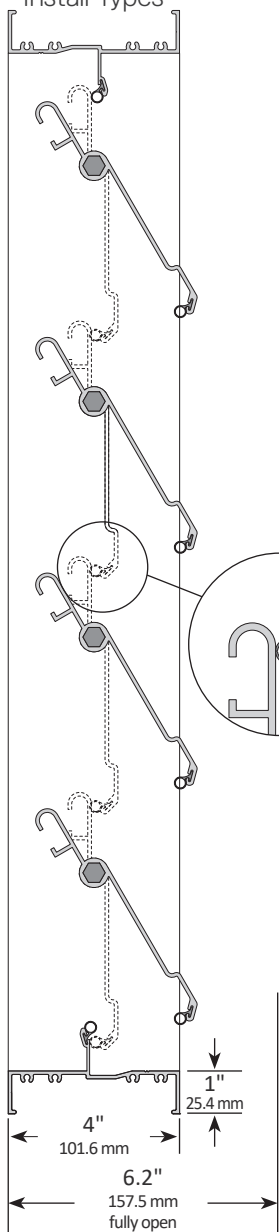
Extended Rear Flange Install Type
